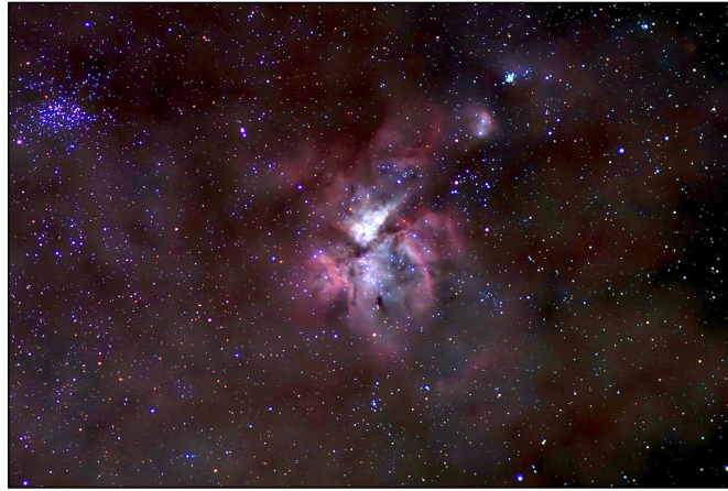
Carina Nebula
