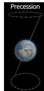
Epoch 1950.0
