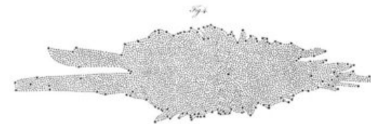
Herschel's structure of the Milky Way (1785)
