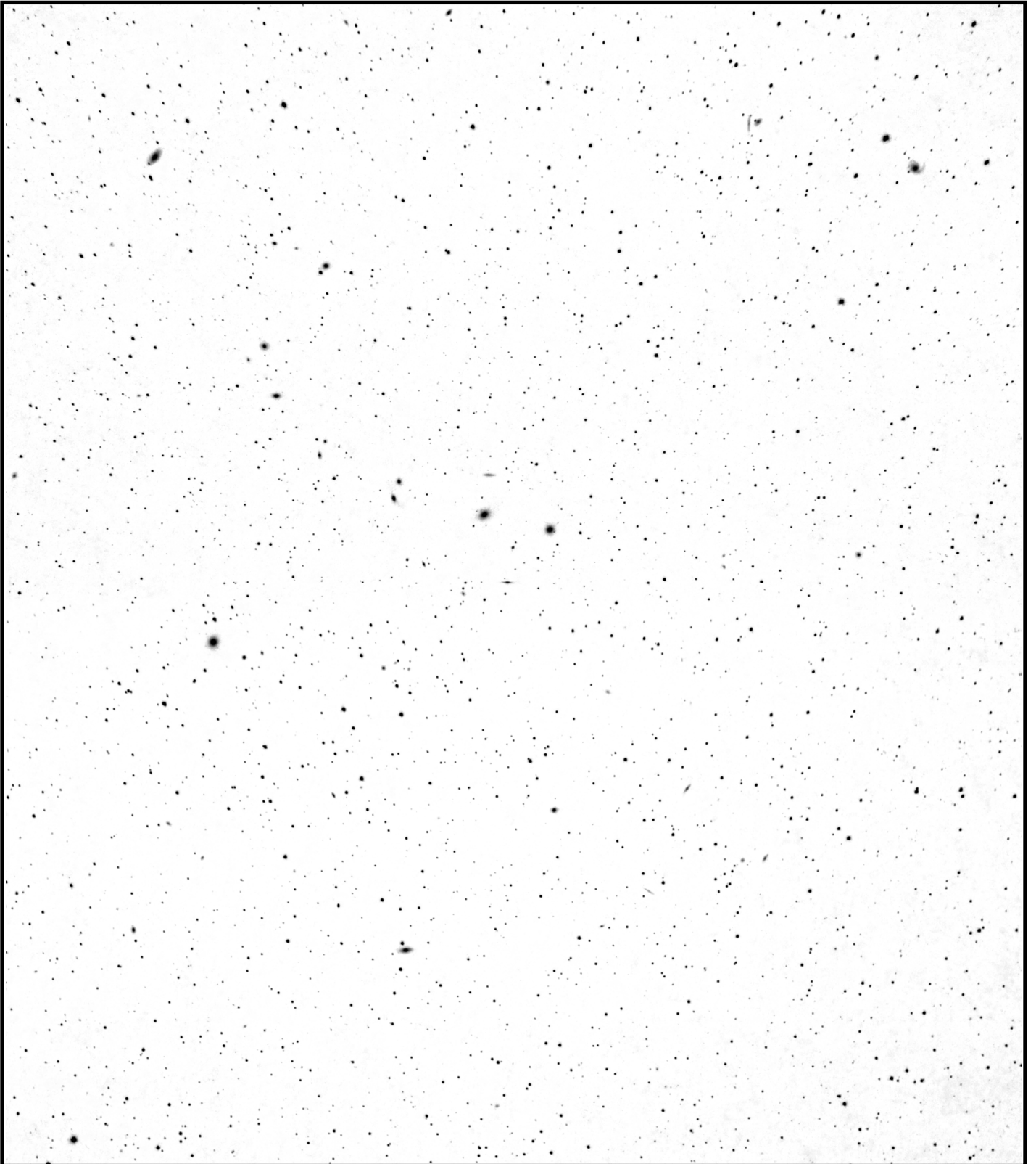
Markarian's Chain and other galaxies in Virgo and Coma Berenices
