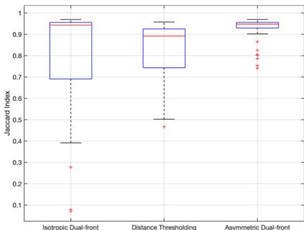
Fig. 9. Box plots of the Jaccard index values on 80 CT image with respect to different models
