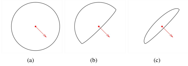
Fig. 1. Unit balls \mathcal{B} for the metrics \mathcal{F} with respect to different tensor fields \mathcal{M} and vector fields \omega , see text. The black lines are the boundaries of \mathcal{B} , the red dots are the origin and the red arrows indicate the orientation \mathbf{p} = (1, -1)^T
