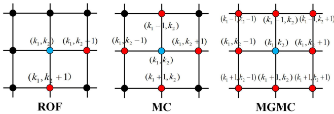
Fig. 11. The illustration of points used to estimate the update for the central point (blue one), where the red points are used for calculation.
