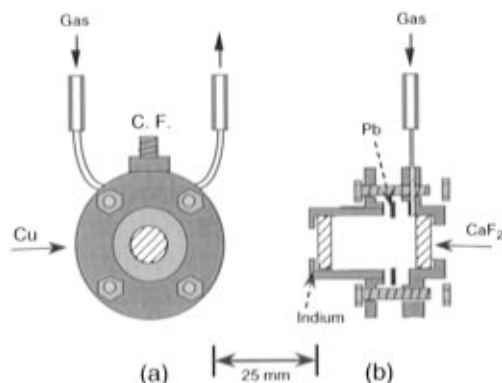
Figure 3. (a) External view and (b) cross-section of the miniature high-pressure IR cell used for the experiments with \text{scCH}_4 . The cell is constructed from copper and is capable of being cooled to cryogenic temperatures. Parts are labelled as follows: (C. F.) mounting stud for cold finger of cryogenic cooler; (Indium) metal seals uniting the \text{CaF}_2 to the Cu cell body; (Pb) main lead seal between the halves of the cell; ( \uparrow and \downarrow ) gas fill ports. Note that this cell has an optical pathlength of ca. 25 mm, much longer than that in the cell shown in Figure 1.
