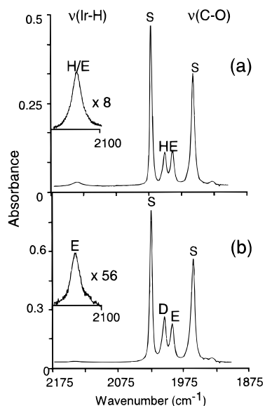
Figure 5. FTIR spectra recorded in scXe after UV irradiation of \text{Cp}^*\text{Ir}(\text{CO})_2 with (a) \text{H}_2 in \text{scC}_2\text{H}_6 and (b) \text{D}_2 in \text{scC}_2\text{H}_6 . In both cases, the reaction products were flushed out of the cell into a second high-pressure cell, using the procedure shown in Figure 2. scXe was then condensed into this second cell, and the products were redissolved. The bands are labeled as follows: (D) \text{Cp}^*\text{Ir}(\text{CO})(\text{D})_2 ; (E) \text{Cp}^*\text{Ir}(\text{CO})(\text{H})(\text{C}_2\text{H}_5) ; (H) \text{Cp}^*\text{Ir}(\text{CO})\text{H}_2 ; (S) unreacted \text{Cp}^*\text{Ir}(\text{CO})_2 . In both spectra the \nu(\text{Ir}-\text{H}) region is shown as an inset with expanded absorbance scale.
