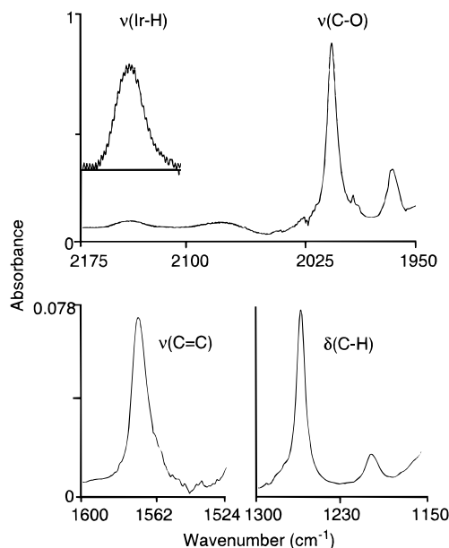
Figure 9. IR spectra, recorded in \text{scXe} , showing the bands of the products of UV irradiation of a solution containing \text{Cp}^*\text{Ir}(\text{CO})_2 in \text{scC}_2\text{H}_4 . As before, the mixtures of products were flushed out of the supercritical cell (see Figure 2); the solids were collected and redissolved in \text{scXe} . Since the \nu(\text{C-O}) bands of \text{Cp}^*\text{Ir}(\text{CO})_2 and \text{Cp}^*\text{Ir}(\text{CO})(\eta^2\text{-C}_2\text{H}_4) overlap, the \nu(\text{C-O}) bands of unreacted \text{Cp}^*\text{Ir}(\text{CO})_2 have been removed from the spectra by scaled computer subtraction. The bands are assigned to \text{Cp}^*\text{Ir}(\text{CO})(\eta^2\text{-C}_2\text{H}_4) , \text{Cp}^*\text{Ir}(\text{CO})(\text{H})(\eta^1\text{-CH=CH}_2) , and \text{Cp}^*\text{Ir}(\eta^2\text{-C}_2\text{H}_4)_2 , as listed in Table 2.
