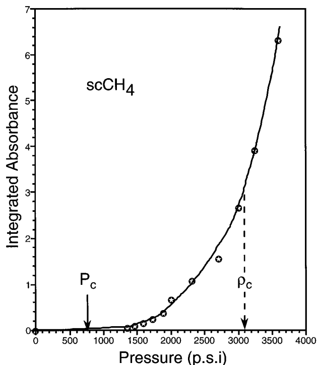
Figure 10. Plot showing the variation in solubility of \text{Cp}^*\text{Ir}(\text{CO})_2 in \text{CH}_4 over a range of gas pressures at 275 K, as measured by the sum of the integrated IR absorbance (arbitrary units) of the two \nu(\text{C}-\text{O}) bands of \text{Cp}^*\text{Ir}(\text{CO})_2 . The integrated rather than peak absorbance was used because the shapes of the bands change as the pressure is increased. Note that \text{Cp}^*\text{Ir}(\text{CO})_2 is virtually insoluble at the critical pressure, P_c (669 psi), but that it increases rapidly when the density of the gas reaches its critical value, \rho_c ( 0.162 \text{ g/cm}^3 ).
