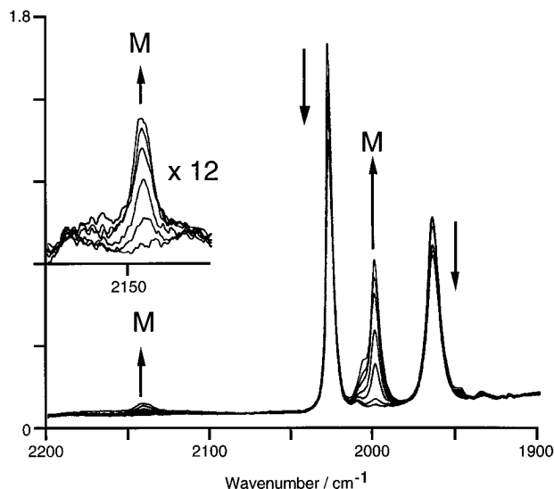
Figure 11. Series of IR spectra, recorded at 5 min intervals, showing the effects of UV photolysis ( >300 \text{ nm} , 30 min total irradiation time) of \text{Cp}^*\text{Ir}(\text{CO})_2 in \text{scCH}_4 at 270 atm pressure and 295 K. The bands of \text{Cp}^*\text{Ir}(\text{CO})_2 are marked \downarrow , those of \text{Cp}^*\text{Ir}(\text{CO})(\text{H})\text{Me} are labeled M. As in previous spectra, the \nu(\text{Ir}-\text{H}) region is shown as an inset with an expanded absorbance scale. The solution is more dilute than in the other fluids, but the absorbance values in these spectra are similar to those in the other figures, because the spectra were recorded with an optical path-length of 25 mm, ca. 10–25 times longer than those used with the other fluids. Note also that the growth of the band of \text{Cp}^*\text{Ir}(\text{CO})(\text{H})\text{Me} is only partially matched by a decrease in intensity of the bands of \text{Cp}^*\text{Ir}(\text{CO})_2 because, unlike the other experiments, this experiment was performed with a saturated solution of \text{Cp}^*\text{Ir}(\text{CO})_2 and more material dissolved during the irradiation.
