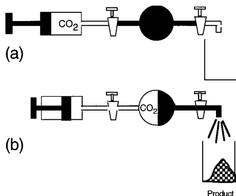
Figure 2. Schematic representation of the procedure for product retrieval from the cell shown in Figure 1. (a) At the end of the reaction, the inlet valve is attached to a Lee Scientific Model 501 syringe pump. (b) This pump forces \text{scCO}_2 through the cell and drives the reaction mixture (colored) out through a Jasco 880/881 back-pressure regulator. As the fluid passes through this regulator, the fluid is expanded in a controlled manner and any product dissolved in the fluid is deposited as shown. A key feature of this method is that high-pressure "stabilizing" conditions are maintained right up to the point of precipitation when the product is deposited by rapid expansion of the fluid.
