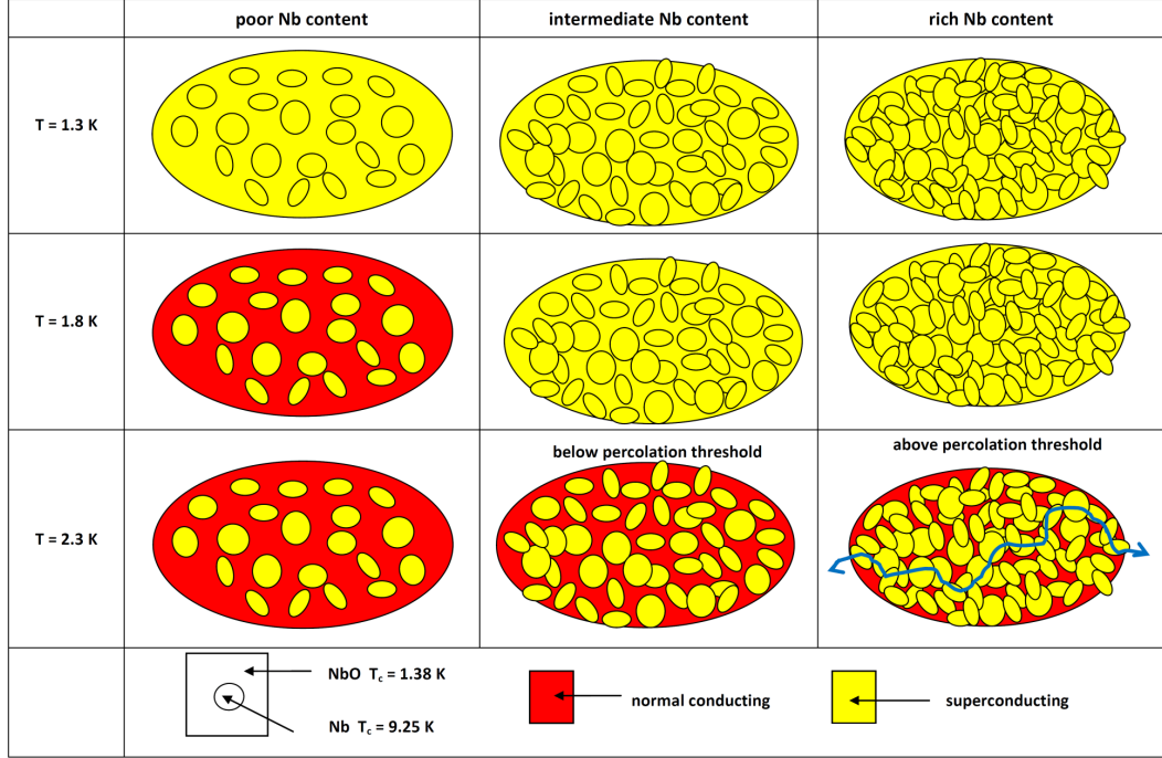
Figure 2.2.: NbO in close contact to niobium. Left: In case of poor niobium content the NbO becomes normal conducting above its transition temperature. Middle: For an intermediate niobium content the whole composite remains superconducting up to a higher temperature by proximity effect. Right: For a sufficiently large niobium content, the niobium is able to form a superconducting paths of its own through the composite. The NbO is now found in the form of small separated normal conducting islands. These islands can serve as condensation nuclei for magnetic flux entry. Courtesy of W. Weingarten.
