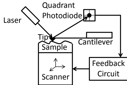
Figure 5.5.: AFM setup following [152].
