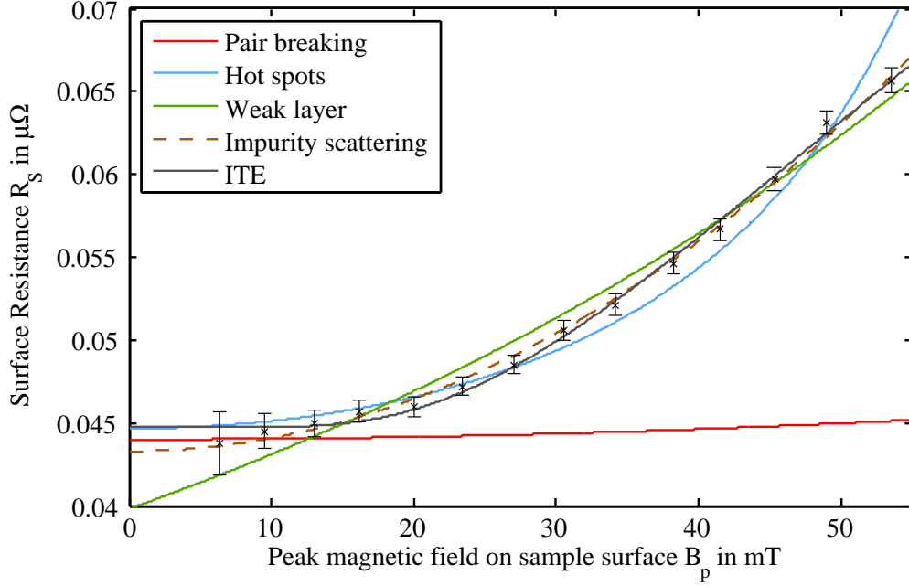
Figure 4.5.: Surface resistance at 400 MHz as a function of applied magnetic field for the clean bulk niobium sample.
