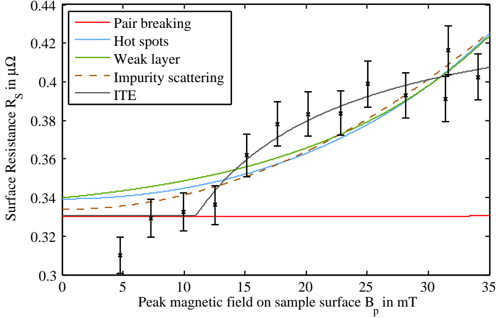
Figure 4.7.: Surface resistance at 400 MHz as a function of applied magnetic field for the niobium film sample.
