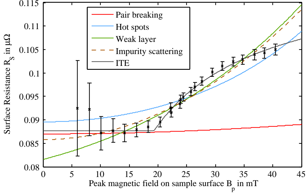
Figure 4.6.: Surface resistance at 400 MHz as a function of applied magnetic field for the dirty bulk niobium sample.
