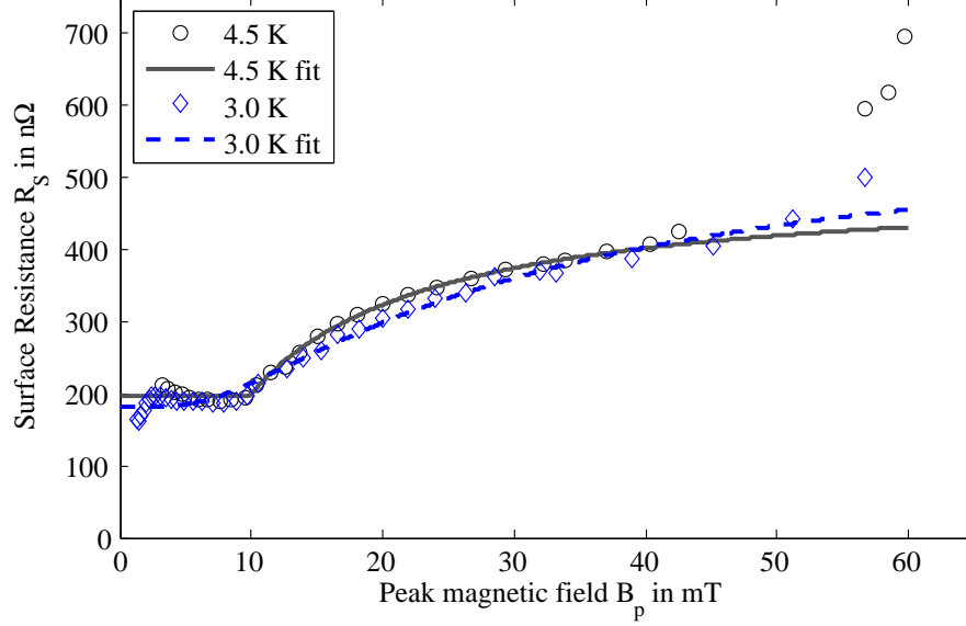
Figure 4.17.: Surface resistance of the HIE Isolde Quarter Wave Cavity at 3 and 4.5 K. The uncertainty is about 10 % for each data point. Measurement performed by M. Therasse and I. Mondino (CERN).
