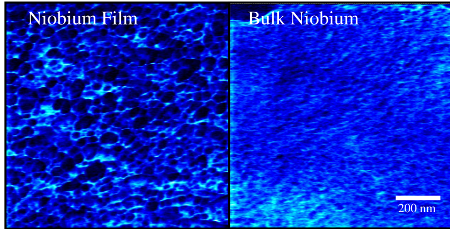
Figure 5.8.: UFM images of the niobium film (left) and the bulk niobium sample (right). A dark (light) color indicate areas of low (high) elasticity. The lateral resolution of the pictures is 4 nm and the surface area displayed is 1 \times 1 \mu\text{m} for each sample. The same surface areas as in Fig. 5.7 are displayed here. Measurements were done in cooperation with Ilya Grishin (University of Lancaster).
