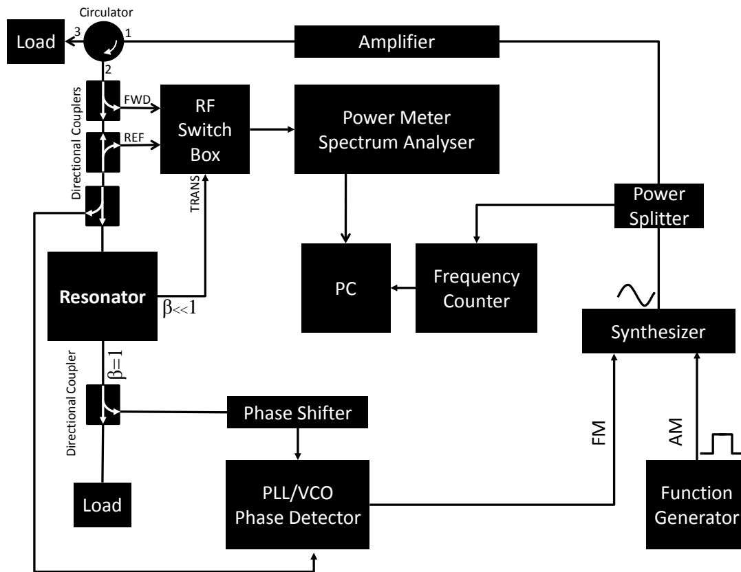
Figure 3.7.: The RF system of the Quadrupole Resonator.
