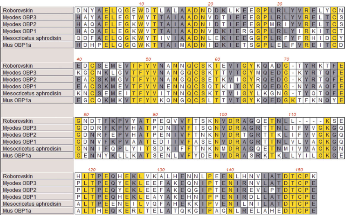
Figure 5 BLAST analysis of the Roborovski hamster urinary protein. The amino acid sequence of the Roborovski hamster urinary protein was used for a BLAST search to identify similar amino acid sequences. The highest match was to urinary olfactory-binding proteins aphrodisin from Myodes glareolus , with strong matches to aphrodisin from Mesocricetus auratus . The isobaric residues leucine (L) and isoleucine (I) were nominated as leucine for the purpose of the BLAST search.
