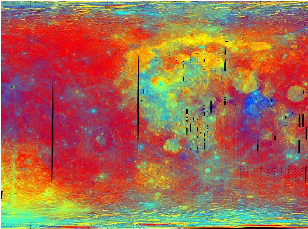
Multispectral false colour image of part of the Moon, showing the geological variation and effects of space weathering processes.
